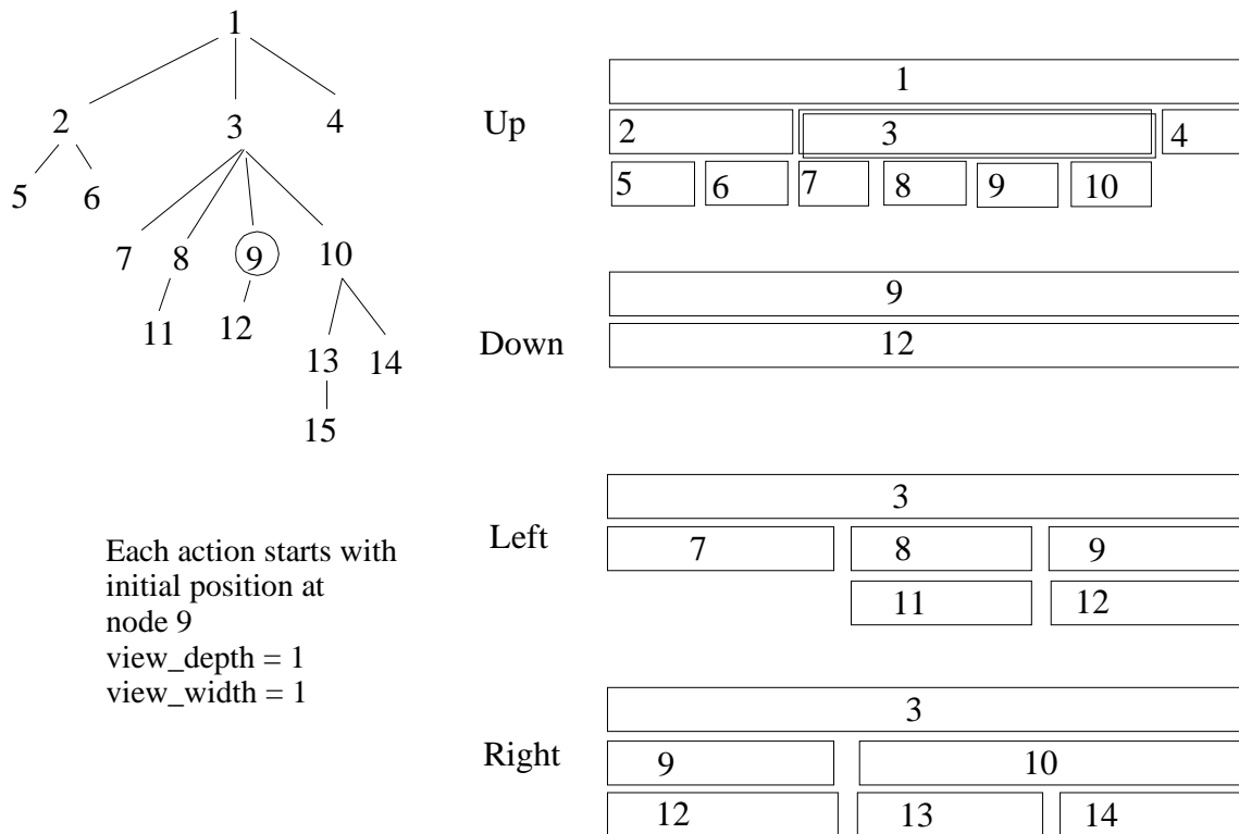
Figure 3 TreeBrowser Actions
